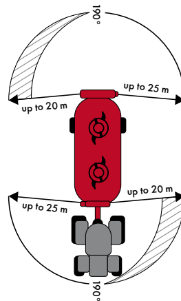
ROTATING, FOLDING TOWER Compact rotating ejector for flexible throwing on all sides.
